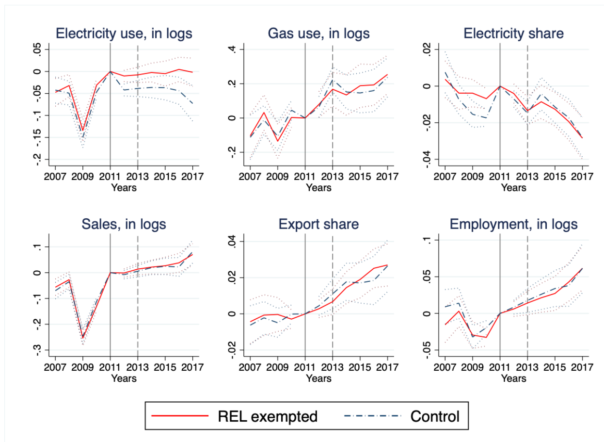
Figure 5: Common trends: Main Matching Specification
