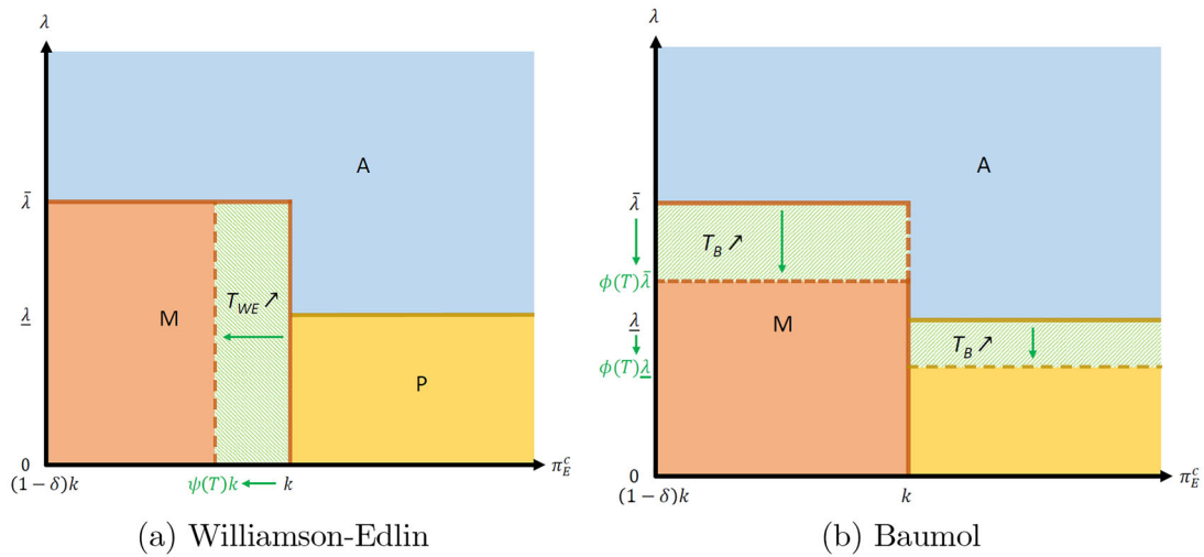
FIGURE 3 | Impact of the Williamson–Edlin and Baumol rules.
