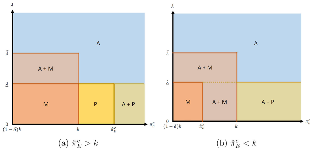
FIGURE 1 | Equilibrium outcomes. A : Accommodation; P : Predation; M : Monopolization.
