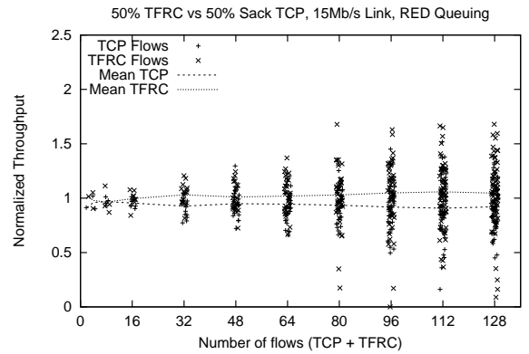
Figure 7: TCP competing with TRFC, with RED.
