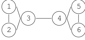
Figure 1: Example tree with d(i) \geq 2, \forall i \in V
