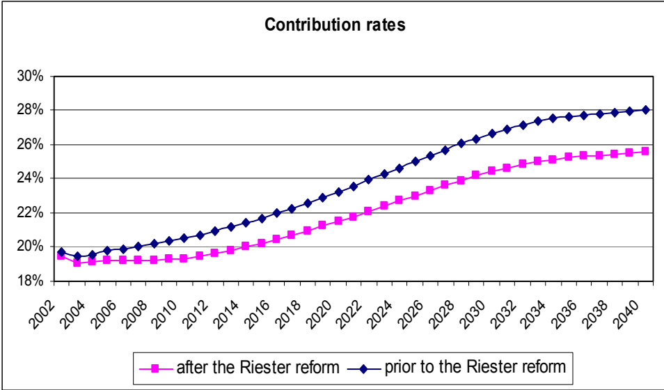
Figure 2-1: Riester formula
