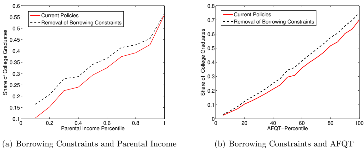
Figure 2: Removing Borrowing Constraints
