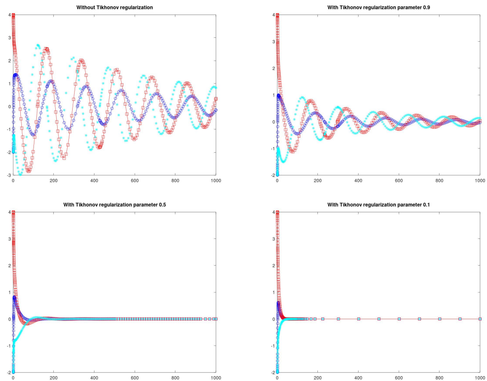
Fig. 6: Trajectories of (FBFR) for regularization parameters \beta \in \{0, 0.1, 0.5, 0.9\} and \gamma = 0.2
