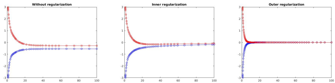
Fig. 2: Trajectories of (FB), (FBIR) and (FBOR) for \lambda = 0.5 and \gamma = 0.15
