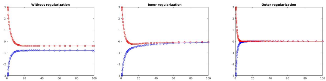
Fig. 3: Trajectories of (FB), (FBIR) and (FBOR) for \lambda = 0.5 and \gamma = 0.3
