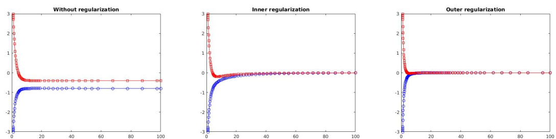
Fig. 5: Trajectories of (FB), (FBIR) and (FBOR) for \lambda = 1 and \gamma = 0.3
