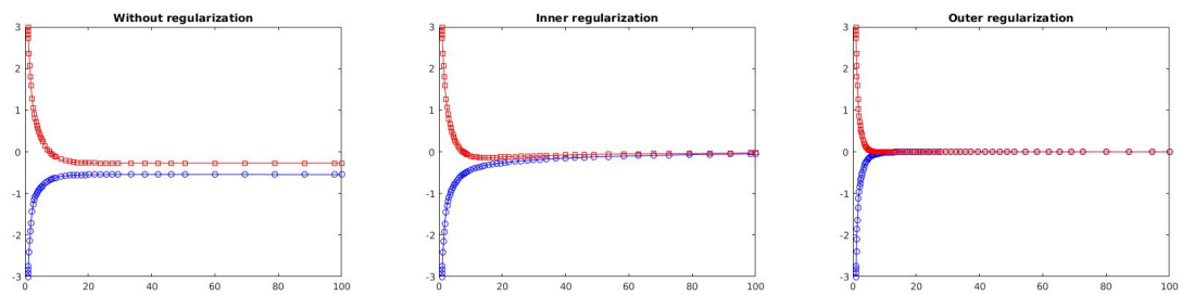
Fig. 4: Trajectories of (FB), (FBIR) and (FBOR) for \lambda = 1 and \gamma = 0.15
