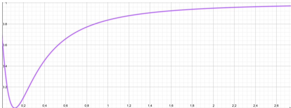
Fig. 1: Graph of \lambda(t) = 0.5 \cos(\frac{1}{0.2+t}) + 0.5
