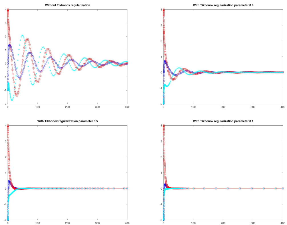
Fig. 7: Trajectories of (FBFR) for regularization parameters \beta \in \{0, 0.1, 0.5, 0.9\} and \gamma = 0.5
