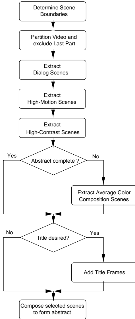
Figure 1: Abstracting Algorithm
